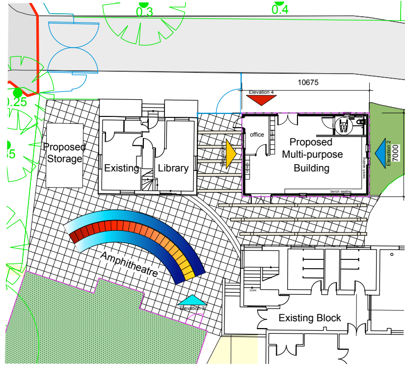
Site Plan (1:100)
